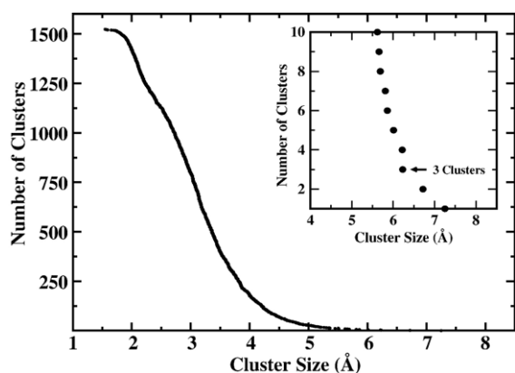
Fig. 6. Number of clusters versus size of the largest cluster. The inset shows abrupt increase in the cluster size for less than three clusters.
