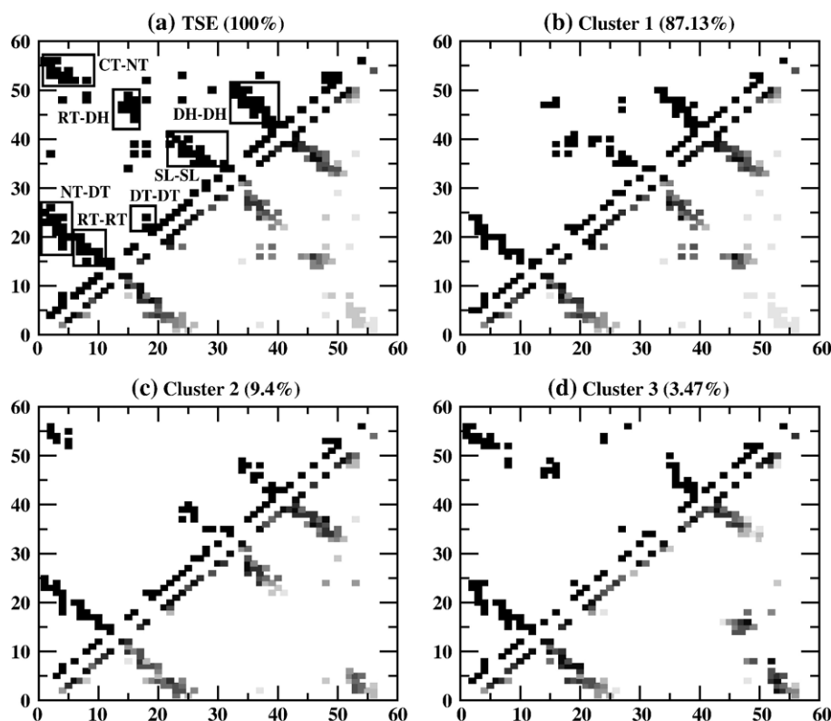
Fig. 1. Contact maps for TSE and clusters. (a) Upper triangle, native contact map. Lower triangle, average contact map of the TSE. (b) through (d) The partition of TSE into three clusters. Upper triangle, contact map of the cluster representative. Lower triangle, average contact map of the cluster. Percentage value on top of the graphs indicates percentage of total TSE.
