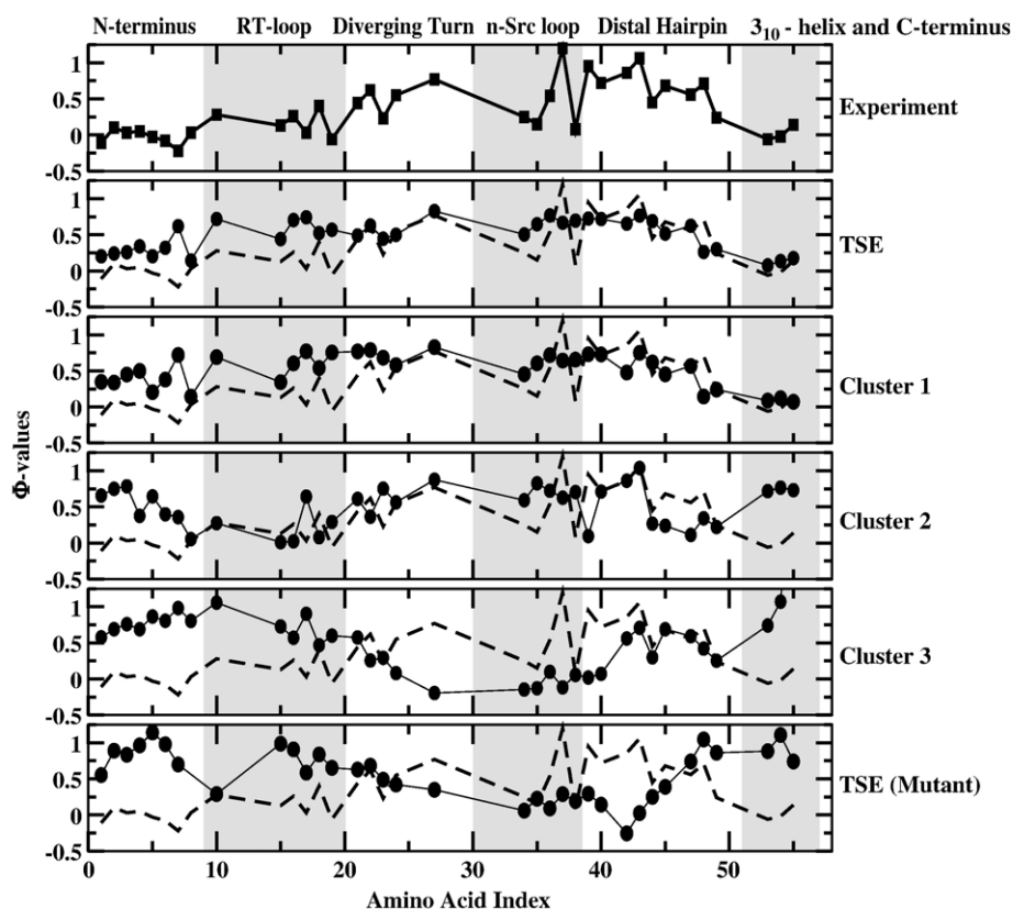
Fig. 2. Experimental (upper panel) and computed \Phi values for the TSE, the three clusters, and the TSE for the mutant. Alternating white and gray boxes differentiate between six consecutive elements of secondary structure labeled at the upper panel. For comparison, we plot the experimental \Phi values in the dashed line.
