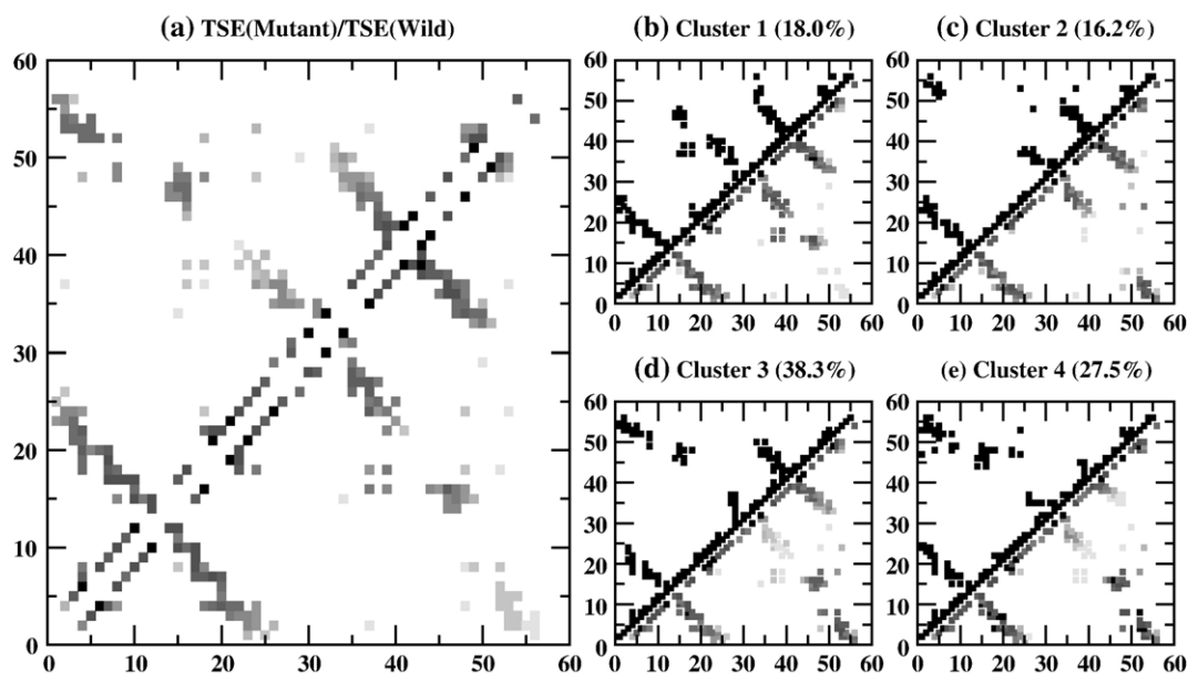
Fig. 3. Contact maps for TSE and clusters after mutation. (a) Lower triangle, average contact map of the TSE before mutation. Upper triangle, average contact map of the TSE after mutation. (b)–(e) Upper triangles, representative of the clusters. Lower triangles, average contact maps of the clusters.
